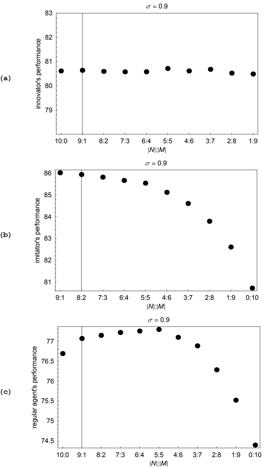
Figure 13: An Average Agent's Performance in Each Group [ \sigma = .9; \rho = 1 ]
