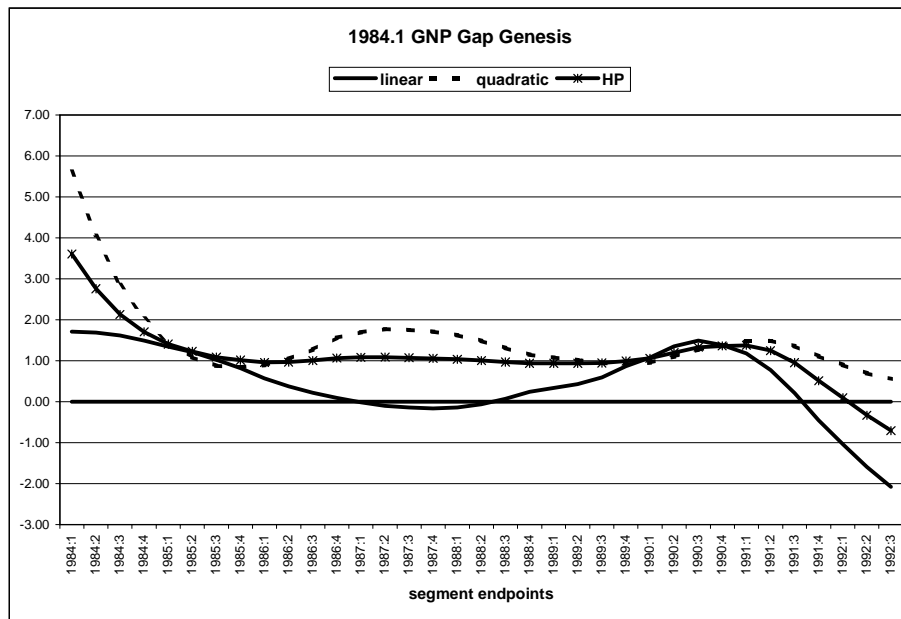
Figure 1: Dependence of Gap Estimates on Future Path Realization
