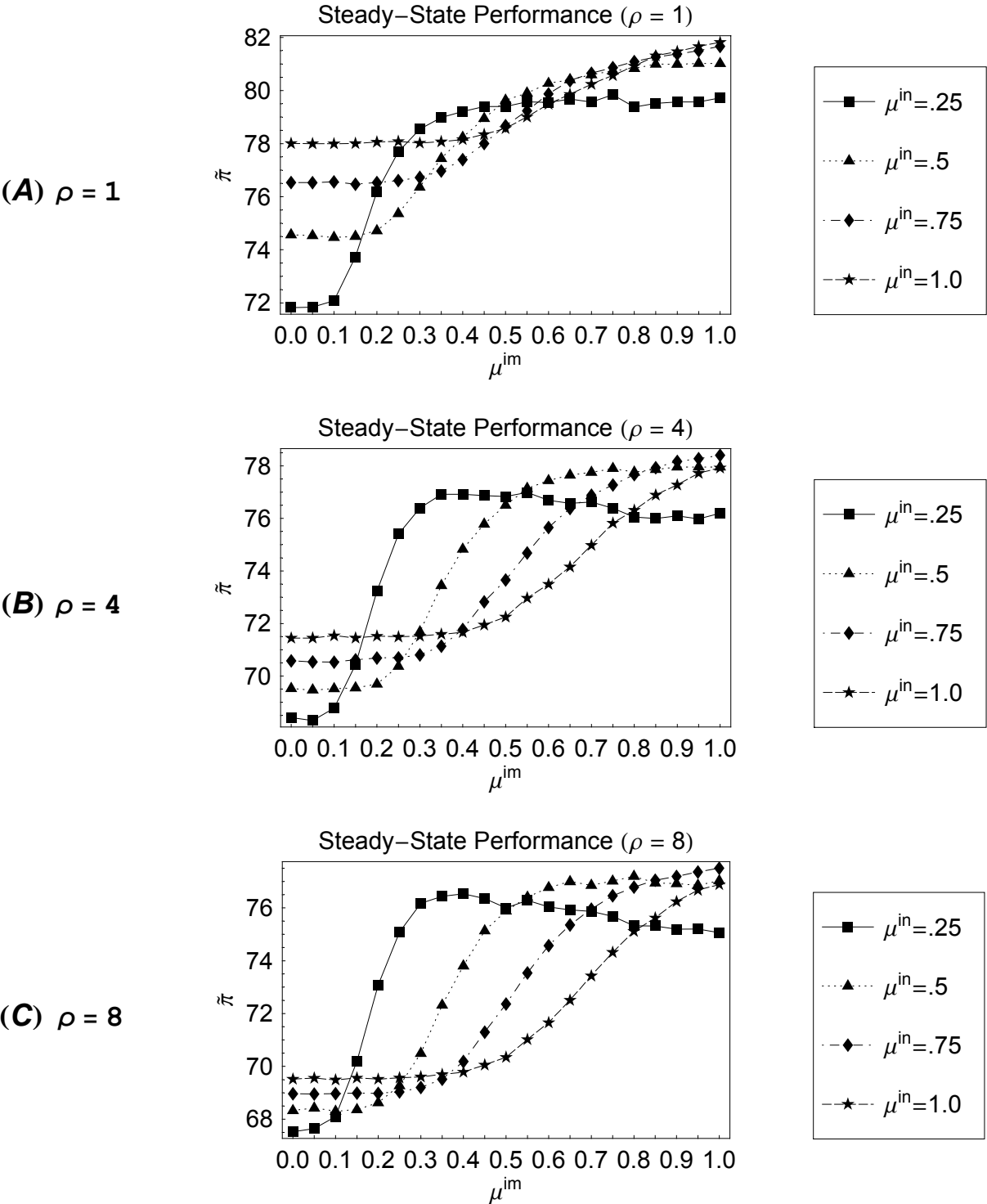
Figure 13: Impact of \rho ( \sigma = .75 ; X = 16 ; \kappa = 16 )
