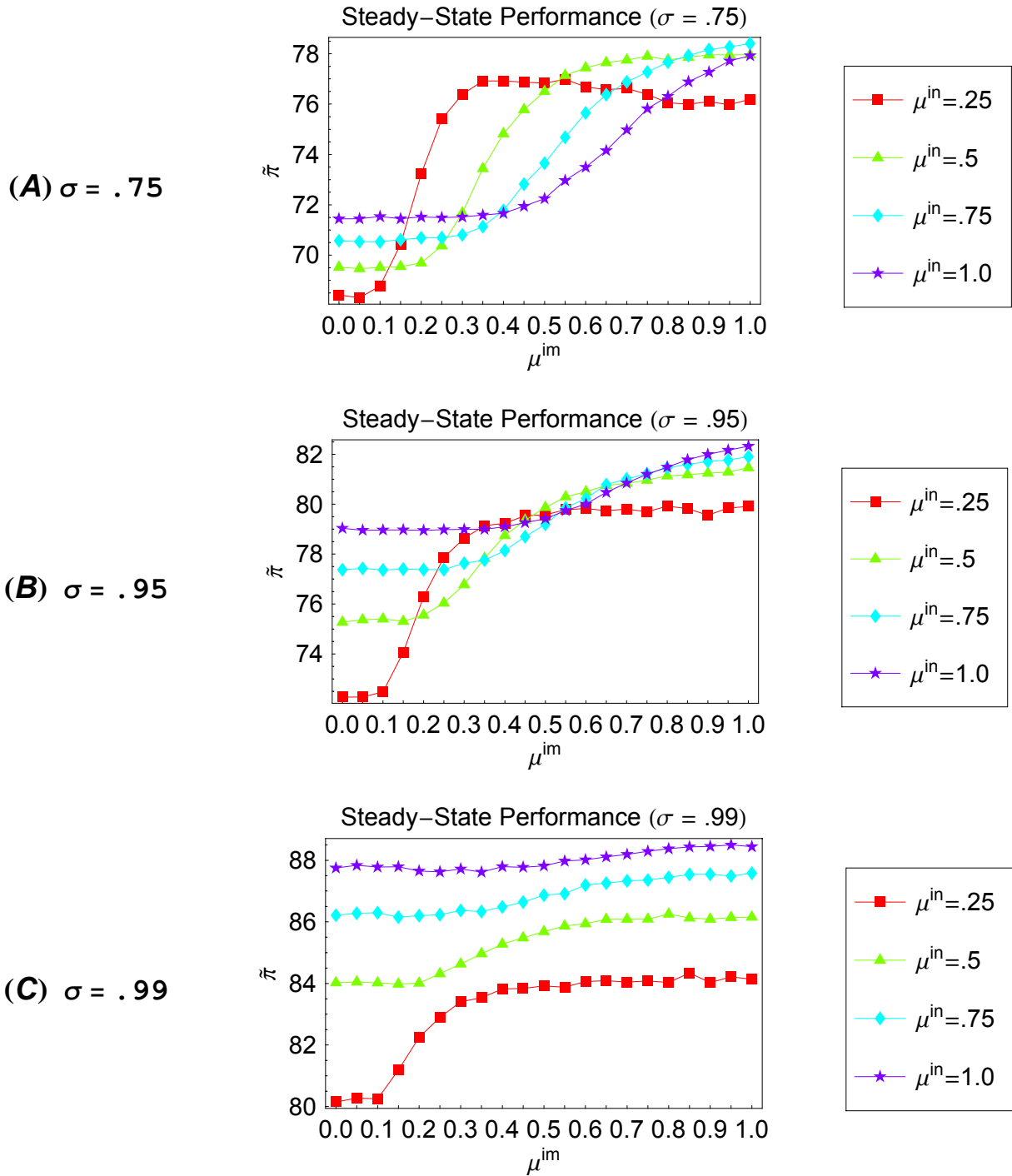
Figure 12: Impact of \sigma ( X = 16 ; \kappa = 16 ; \rho = 4 )
