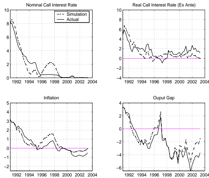
FIG. 11. Higher \mu_\pi
