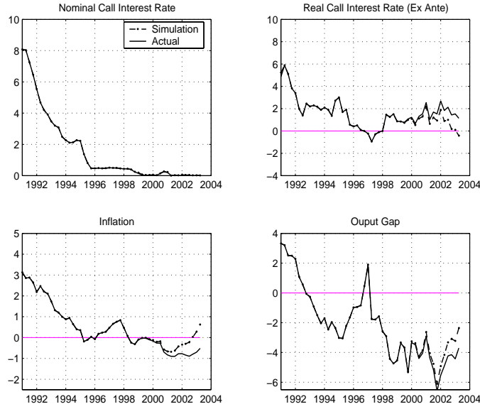
FIG. 13. Nonlinear Policy
