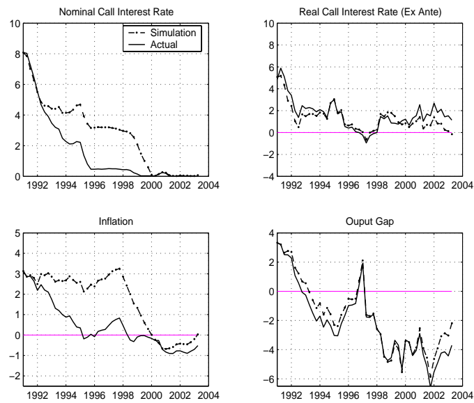
FIG. 10. Higher \pi^*
