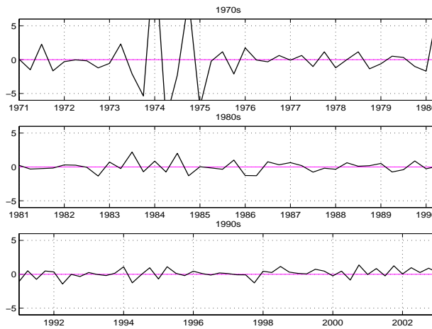
FIG. 7. Inflation Shocks
