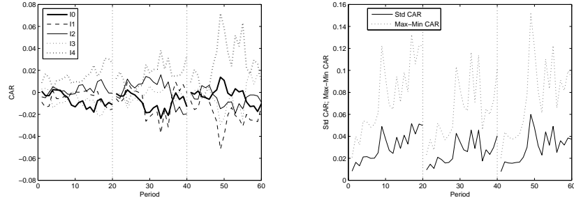
Figure 4: Cumulative abnormal returns of each information level, CAR_{j,r,k} , over periods and repetitions (left panel). The standard deviation ( STD\_CAR ) out the CAR 's and the difference between the maximum and the minimum of the CAR -functions ( MAX - MIN\_CAR ) over time are provided in the right panel.
