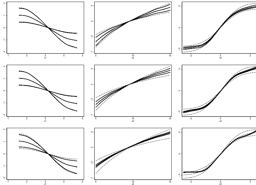
Figure 3: The average estimates of 250 replications (solid) and the true effects (dashed) (1 + \gamma_j) f_j(X_j) for the signal-to-noise ratio 3, 2 and 1 in the first, second and third row, respectively.
