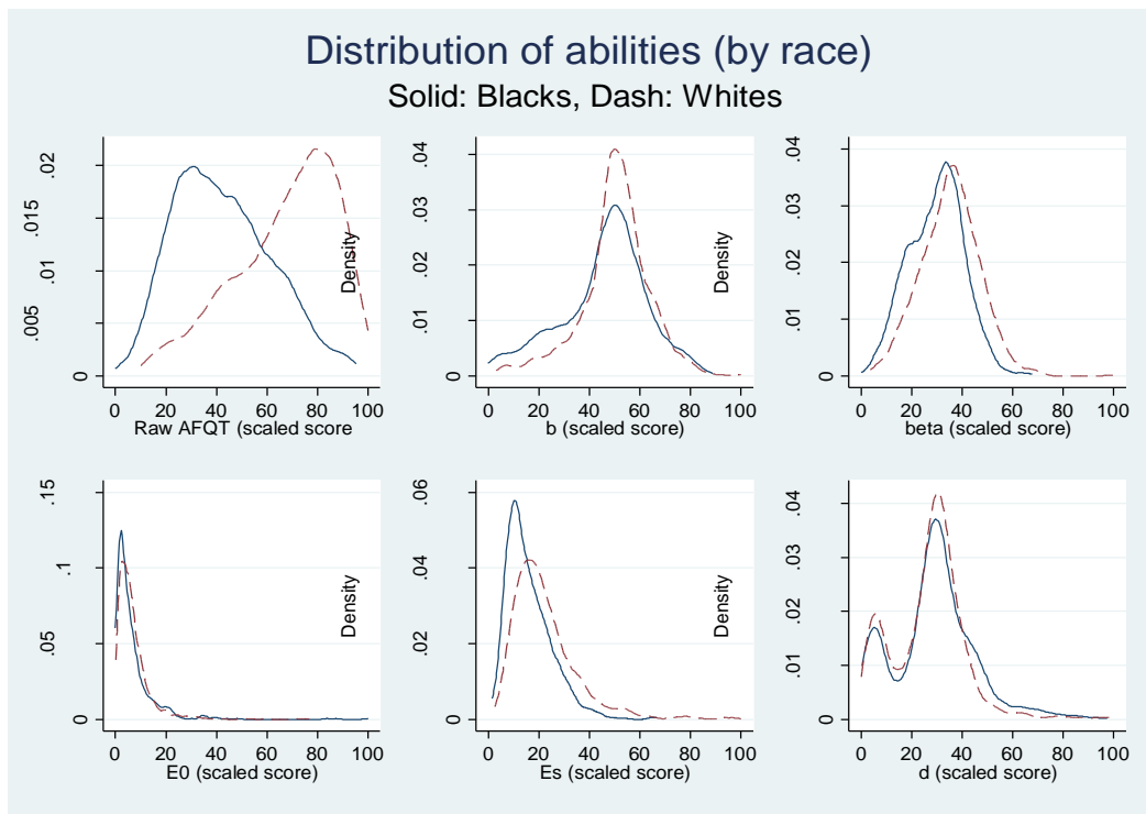
Figure 4 Distribution of Parameter Values*
