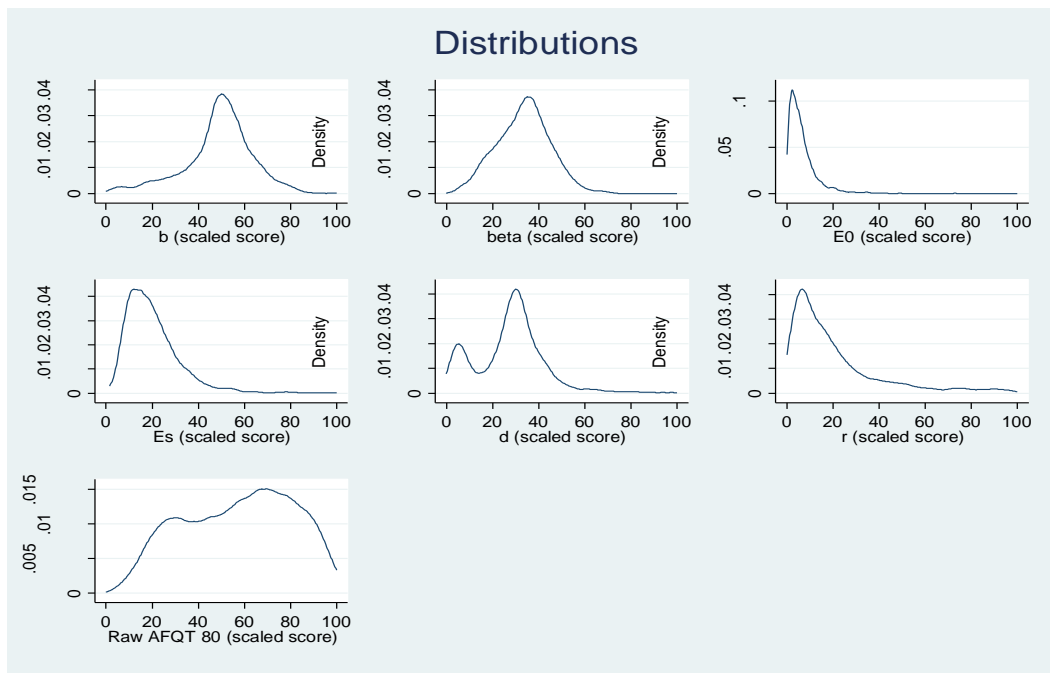
Figure 3 Distribution of Parameter Values*
