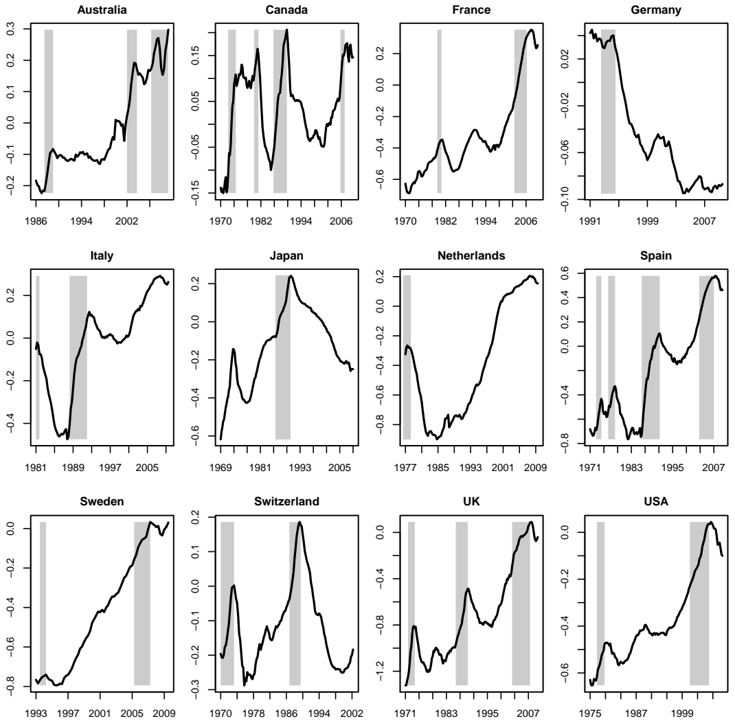
Figure 2: Chronology of the house price bubbles
