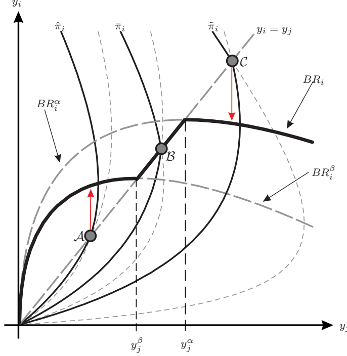
Figure 1 Best response function in the presence of distributional preferences
