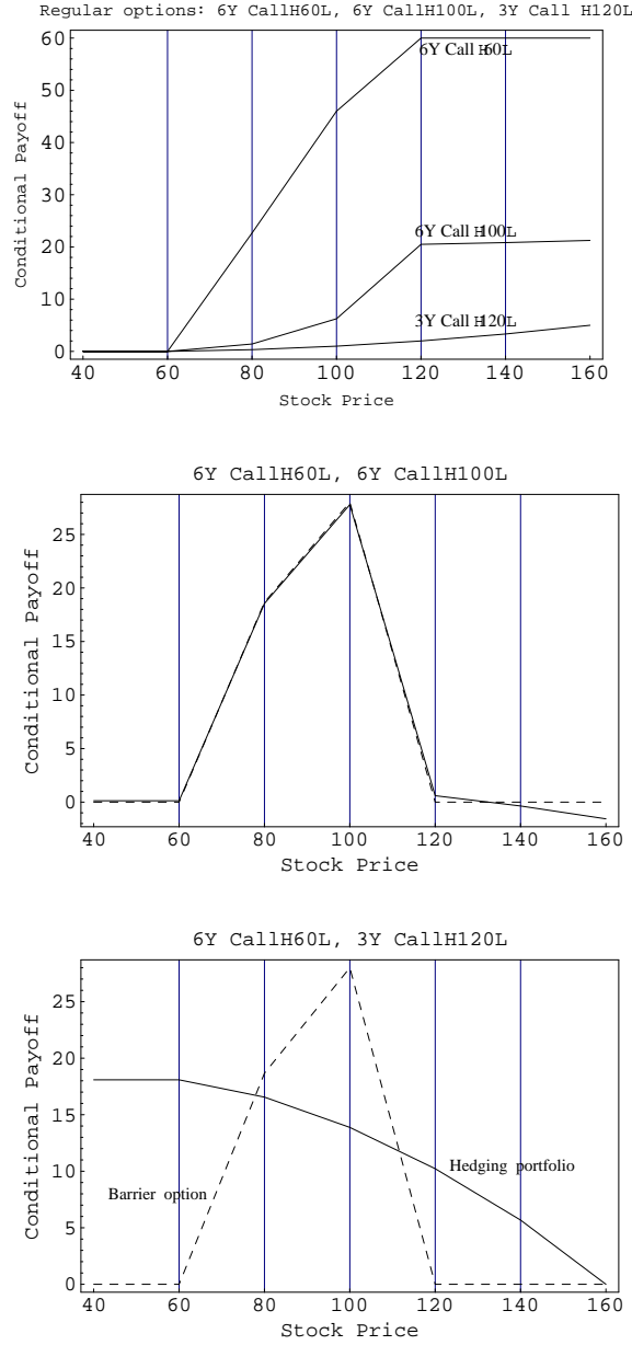
Figure 3: Static hedging strategies allowing liquidation. Conditional values at maturity of the regular options potentially available for hedging (upper panel), of the barrier option and of the hedging portfolio when the short-term option is excluded (middle panel), and when the long-term option with the highest strike is excluded (lower panel).
