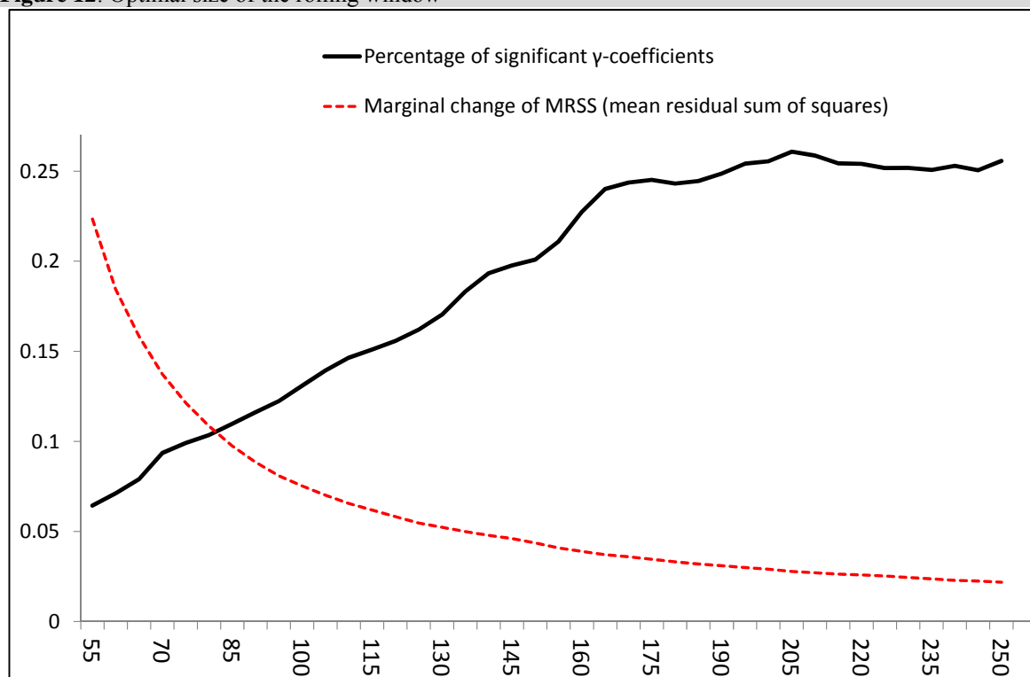
Figure 12: Optimal size of the rolling window
