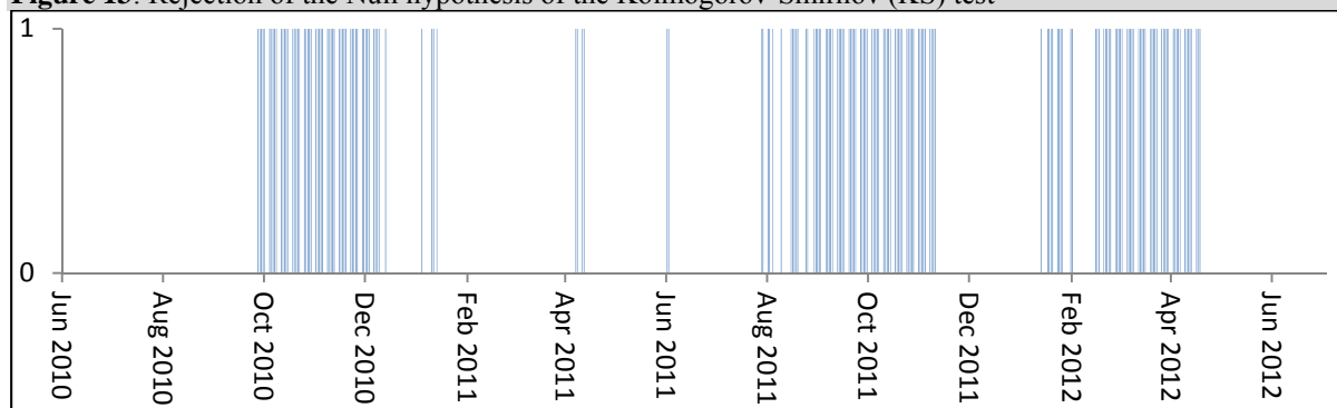
Figure 13: Rejection of the Null hypothesis of the Kolmogorov-Smirnov (KS) test
