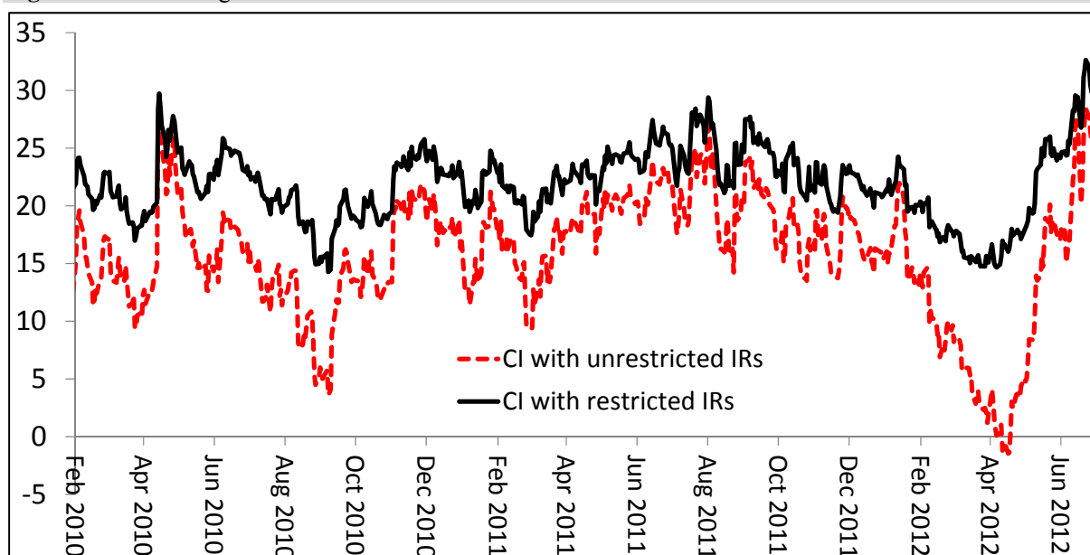
Figure 15: The Contagion Index with restricted and unrestricted IRs
