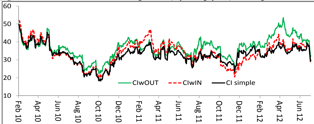
Figure A3.1: Different versions of the EA Contagion Index (in percentage points) of sovereigns
