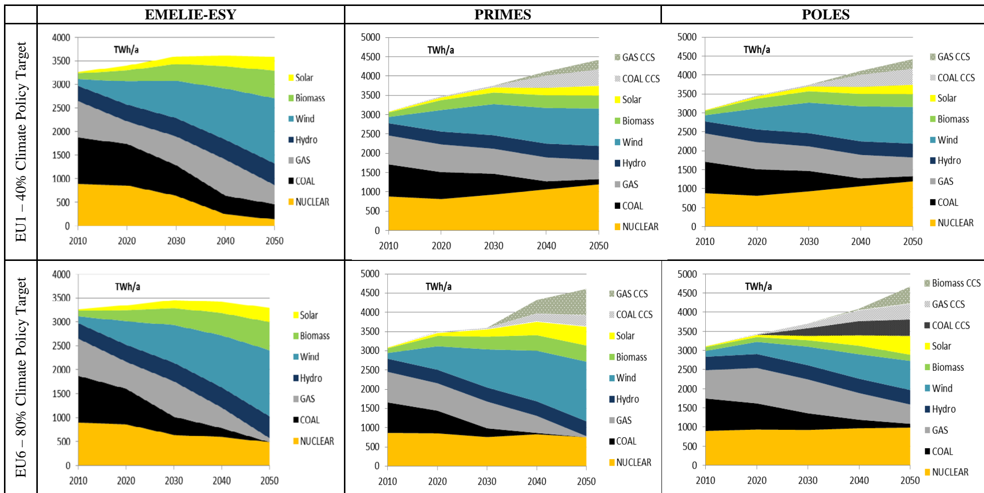
Figure 5: Power Generation of EU-27 (Source: Own compilation)
