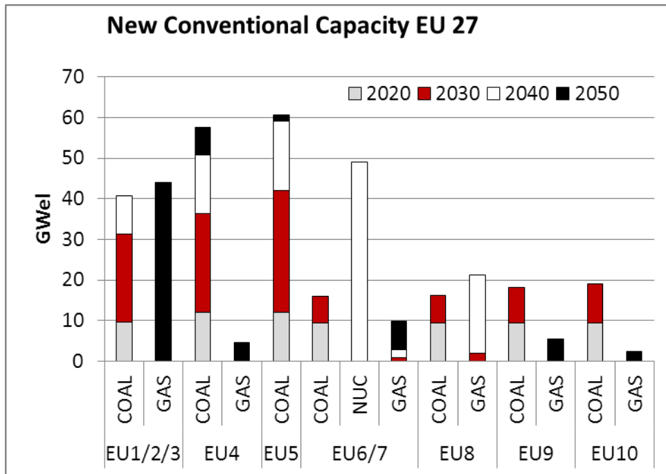
Figure 4: Conventional Capacity Investments until 2050 [GW el net Capacity] (Source: Own illustration)
