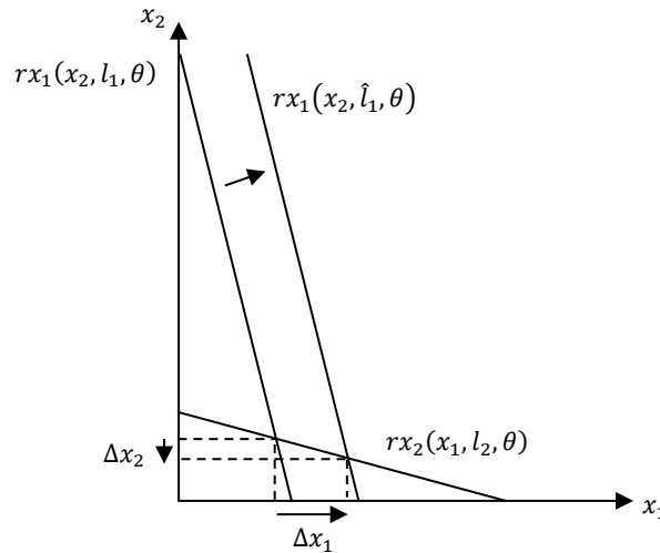
Figure 1: Strategic overinvestment in permits (exemplary for firm i = 1 , where \hat{l}_1 > l_1 ) 22
