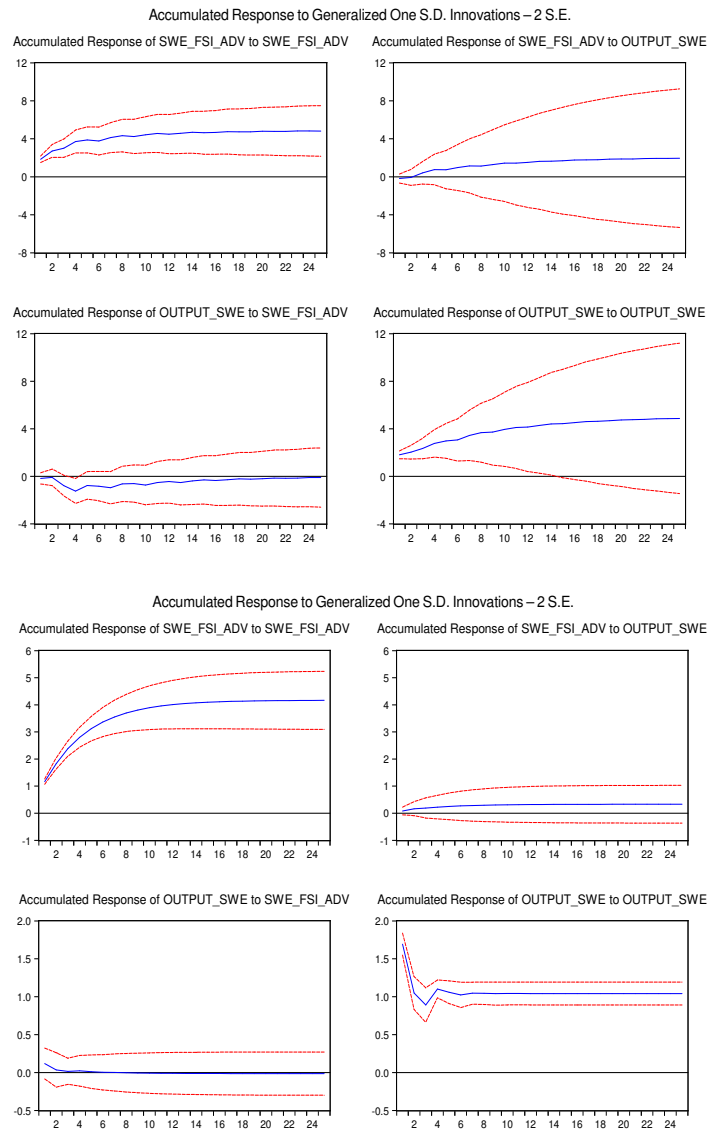
Figure 11: Sweden Multi Regime VAR
