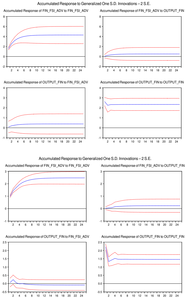
Figure 9: Finland Multi Regime VAR
