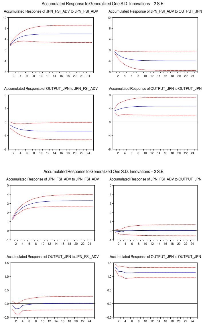
Figure 17: Japan Multi Regime VAR
