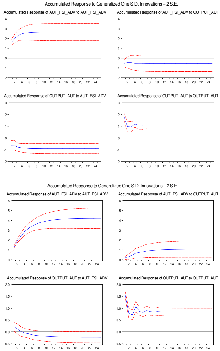
Figure 14: Austria Multi Regime VAR
