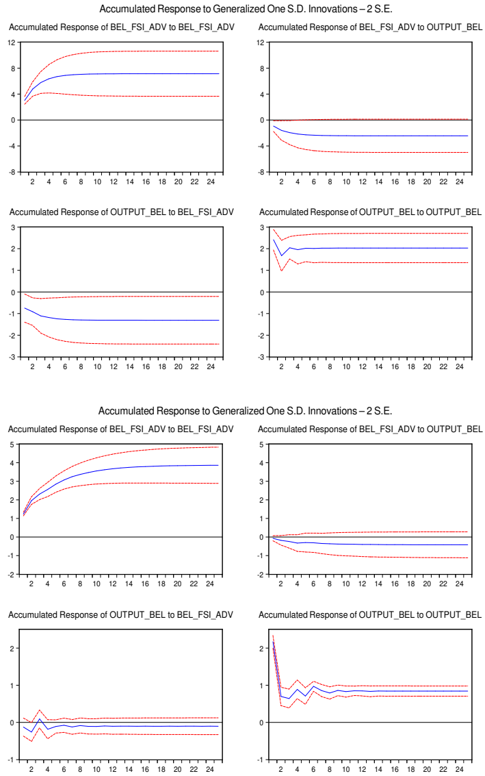
Figure 13: Belgium Multi Regime VAR
