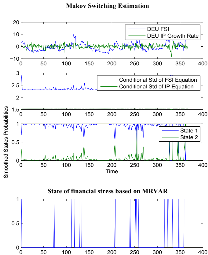
Figure 20: Comparison between MRVAR and Markov Switching for Germany
