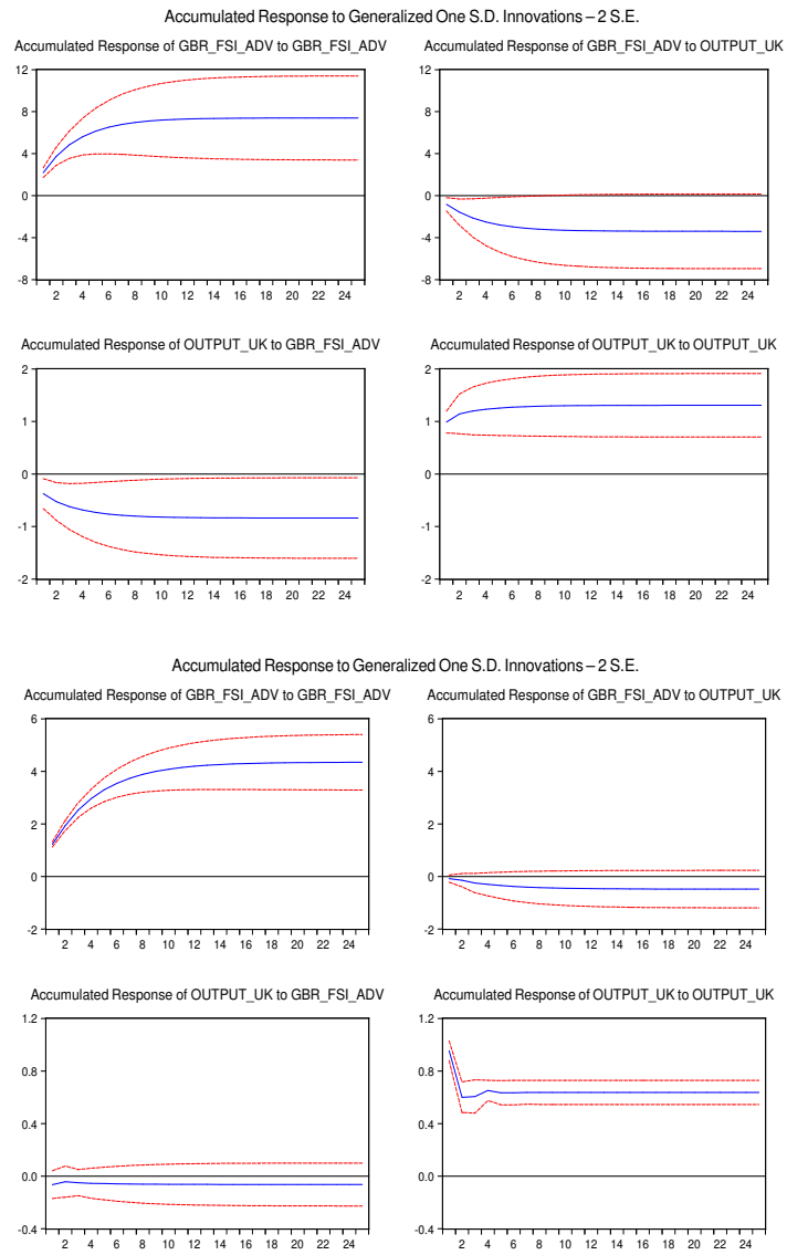
Figure 10: United Kingdom Multi Regime VAR
