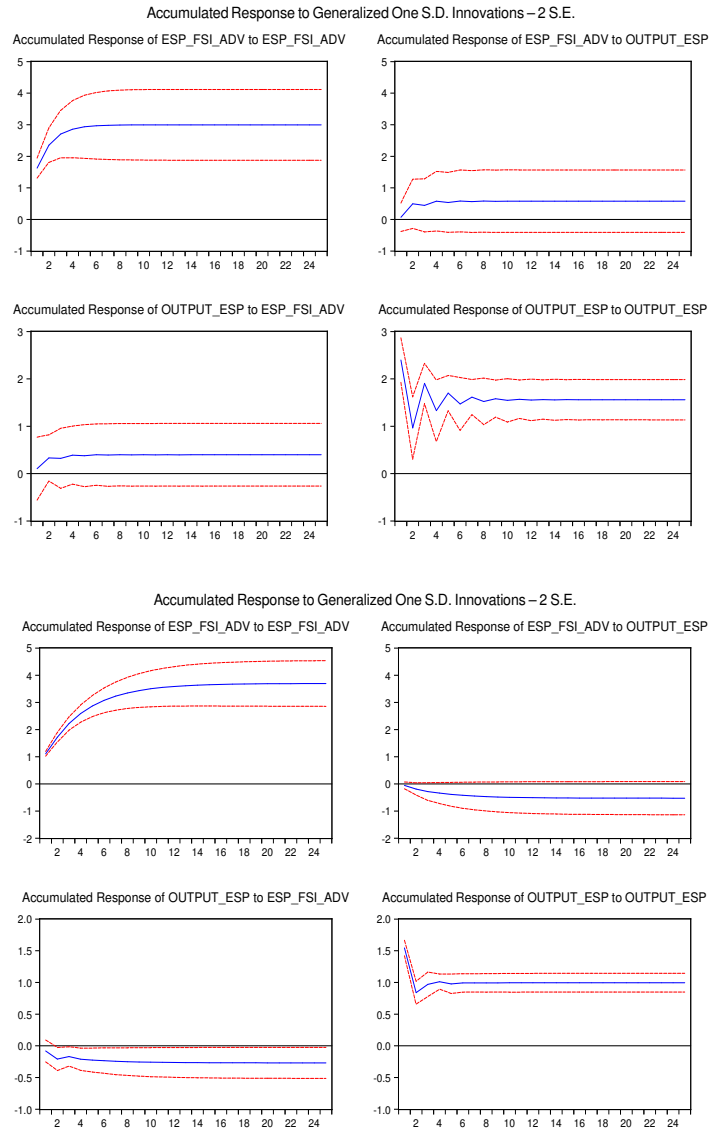
Figure 8: Spain Multi Regime VAR
