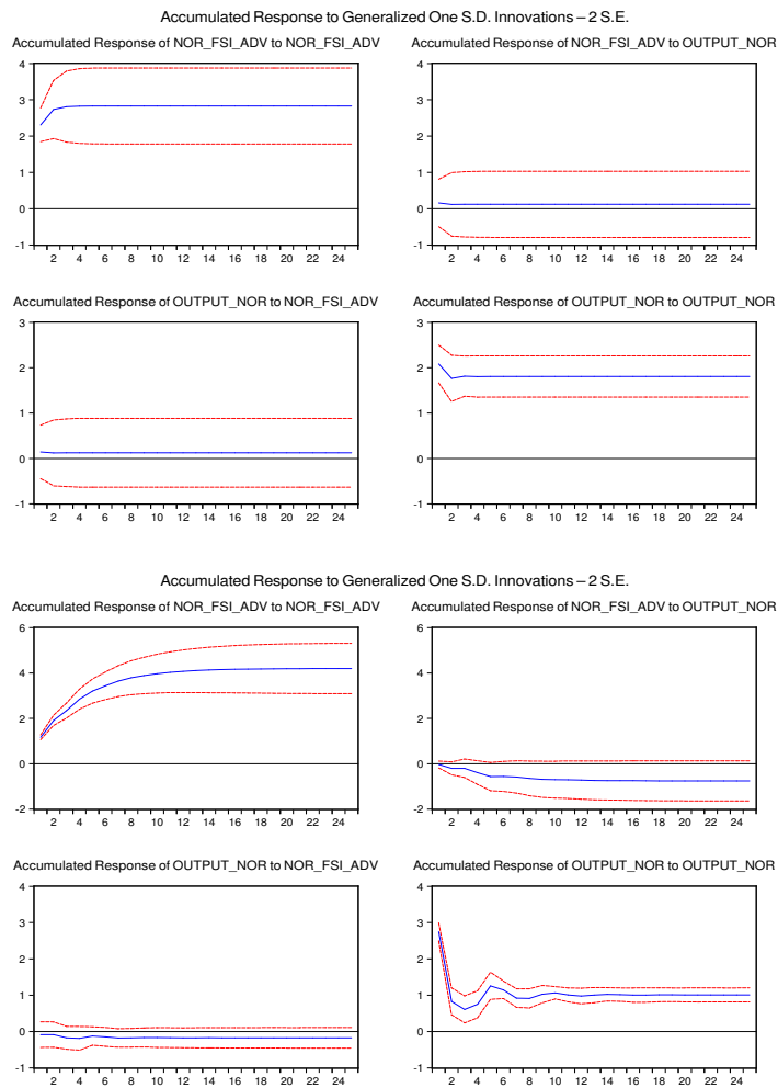
Figure 18: Norway Multi Regime VAR
