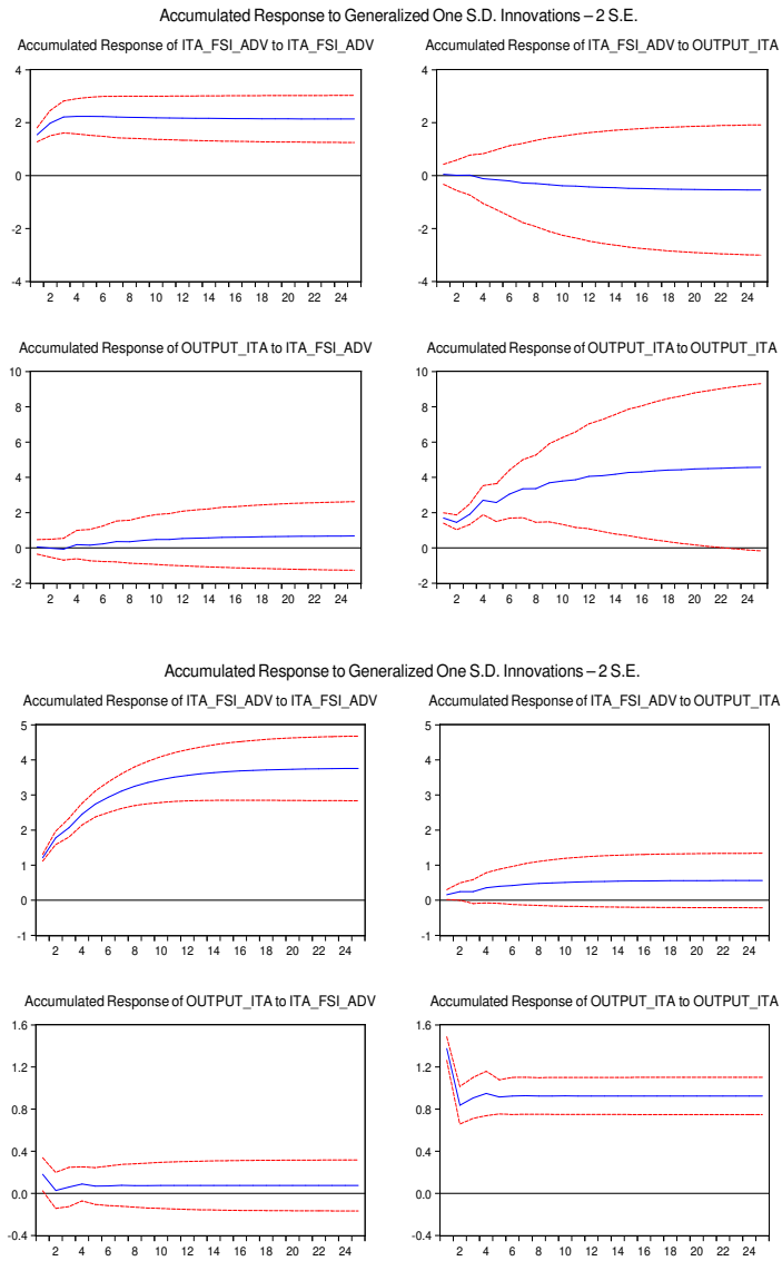
Figure 15: Italy Multi Regime VAR
