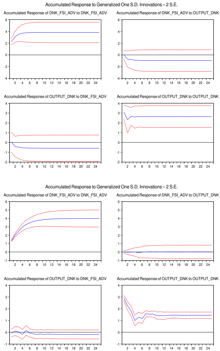
Figure 12: Denmark Multi Regime VAR
