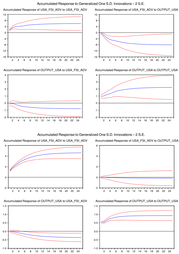
Figure 5: USA Multi Regime VAR
