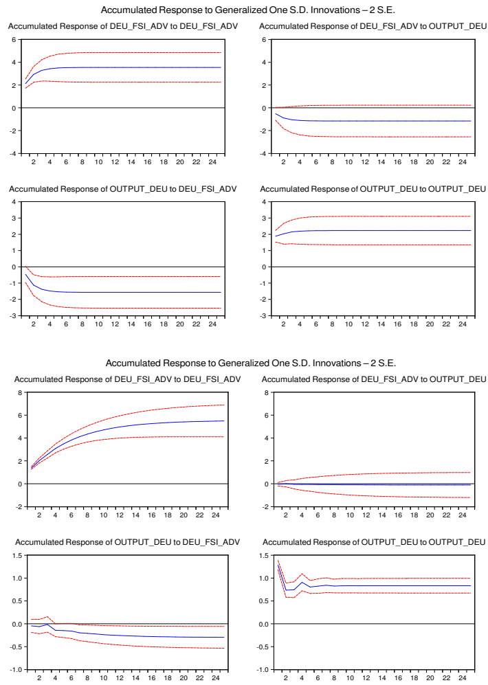
Figure 6: German Multi Regime VAR
