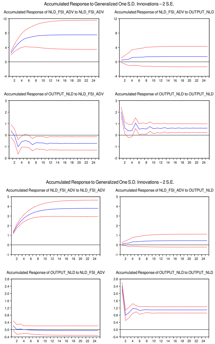
Figure 16: Netherlands Multi Regime VAR
