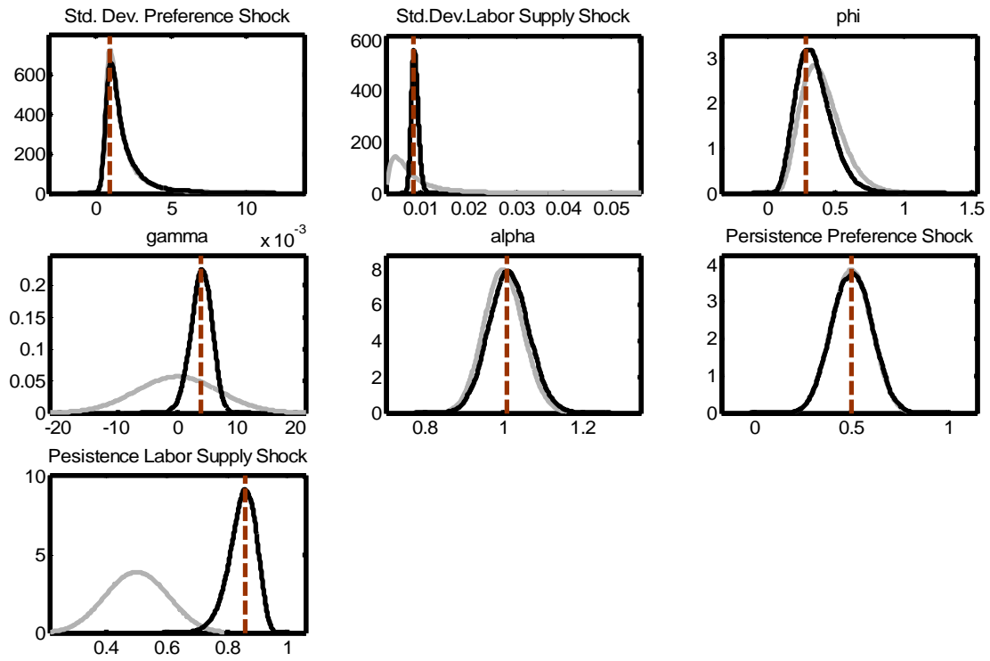
Figure 1. Prior (grey line) and posterior (black line) distribution, and posterior mode (red dashed line) of the estimated parameters of the unconstrained model.
