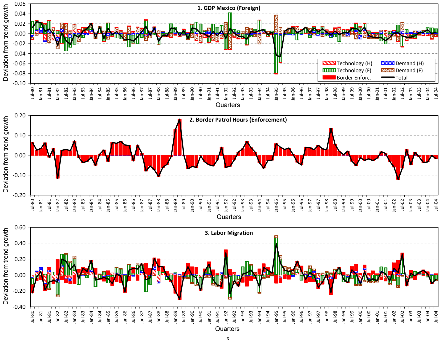
Figure 7. Historical decomposition
