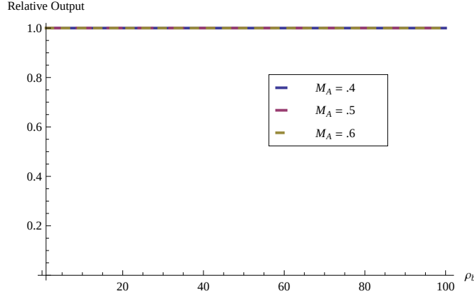
Figure 8: Type A discover potential buyers more frequently: \rho_s = 1 , Varying \rho_b
