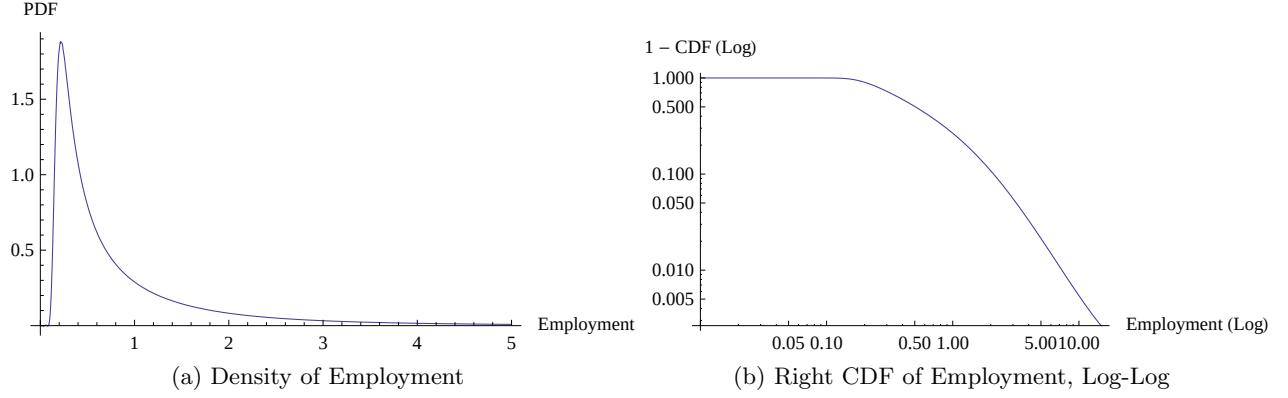
Figure 4: The Distribution of Employment
