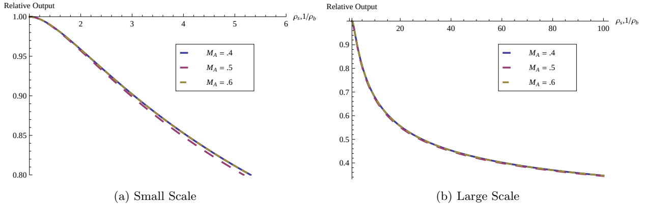
Figure 5: Specialization: Varying \rho_s > 1 , \rho_b < 1
