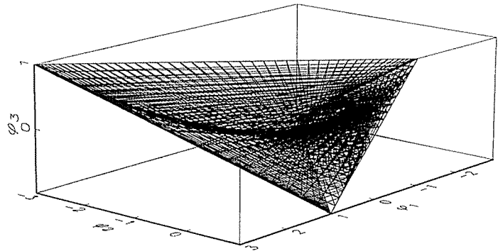
The coefficients stability region S_3
