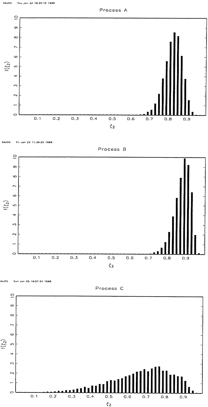
FIGURE 3. Frequency histograms of the probability distribution of \zeta_2 for T = 100 .
