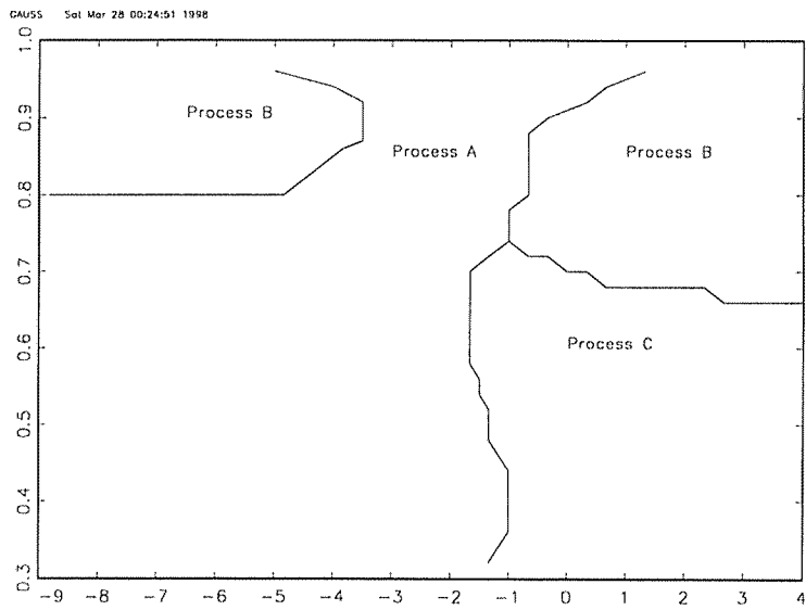
FIGURE 5D. Optimal decision for prediction loss and T = 200 .
