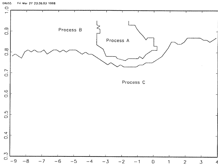
FIGURE 4D. Optimal decision for double-squared loss and T = 200 .
