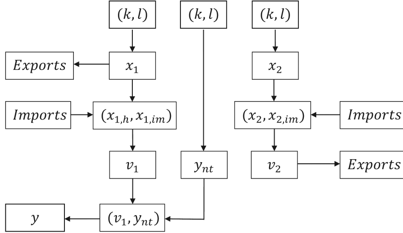
FIGURE 5. MODEL FLOWCHART
