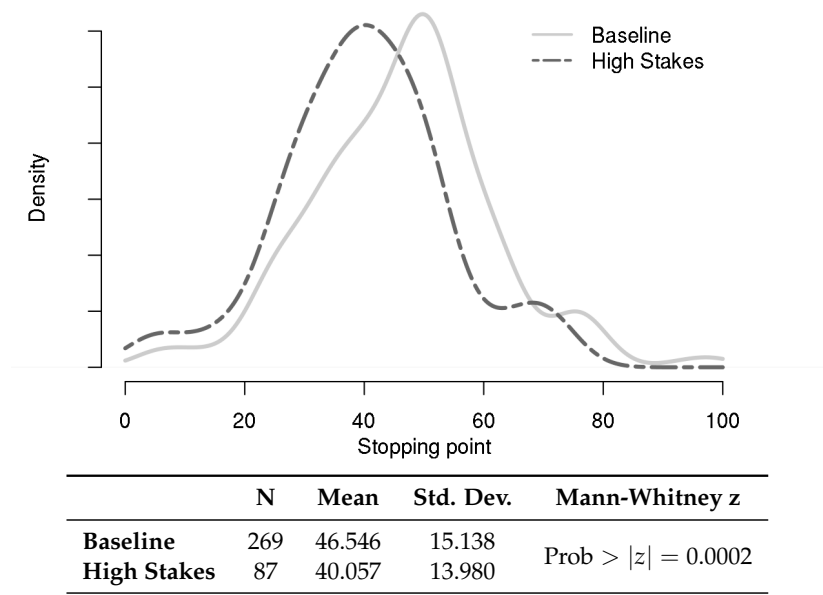
Figure 7: Results and kernel density of decision by treatment, Baseline vs. High Stake
