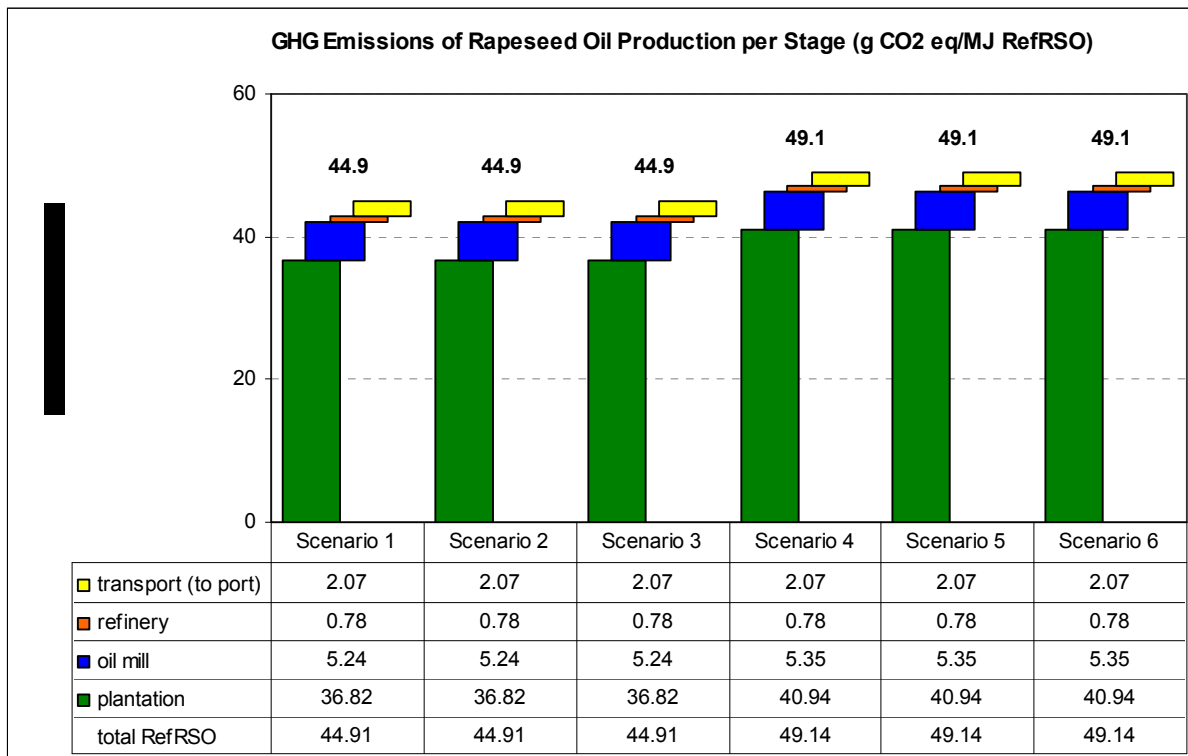
Figure 1: GHG Emissions of refined Rapeseed Oil Production per Stage
