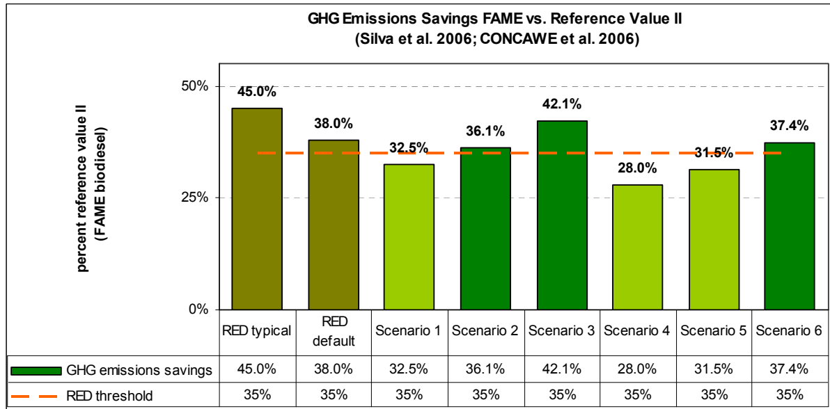
Figure 5: GHG Emissions Savings of Rapeseed FAME (fossil comparator II)
