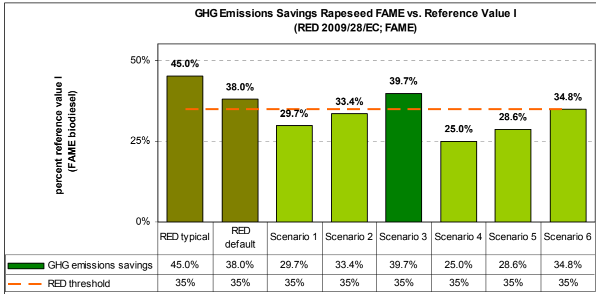
Figure 4: GHG Emissions Savings of Rapeseed FAME (fossil comparator I)
