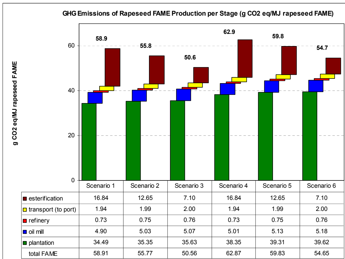
Figure 3: GHG Emissions of Rapeseed FAME Production per Stage
