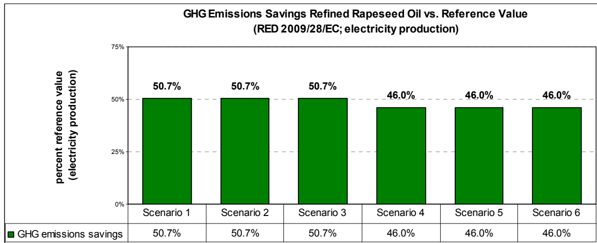
Figure 2: GHG Emissions Savings of refined Rapeseed Oil used in Oil fired Power Plants
