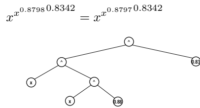
Figure 13: Best candidate frontier s_{\omega(1),3} in generation \mathcal{P}_3
