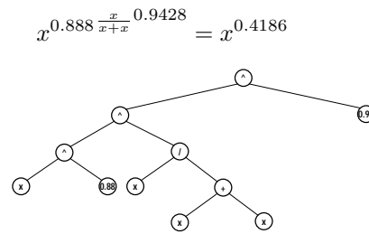
Figure 14: Best candidate frontier s_{\omega(1),4} in generation \mathcal{P}_4
