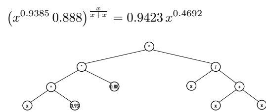
Figure 16: Best candidate frontier s_{\omega(1),17} in generation \mathcal{P}_{17}
