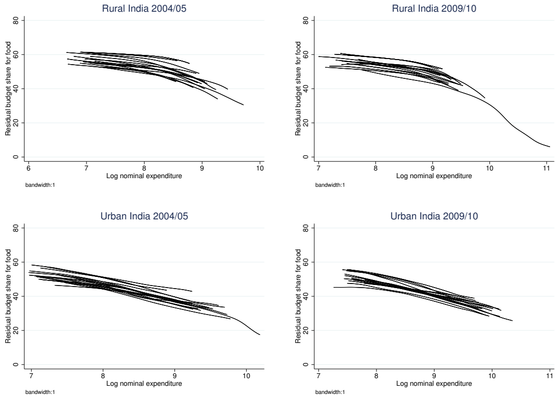
FIGURE 1: Semi-parametric analysis
