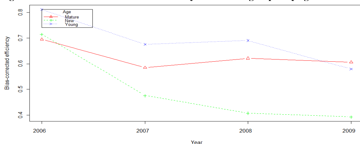
Fig.4 Evolution of the bias-corrected efficiency of the MFIs grouped by age
