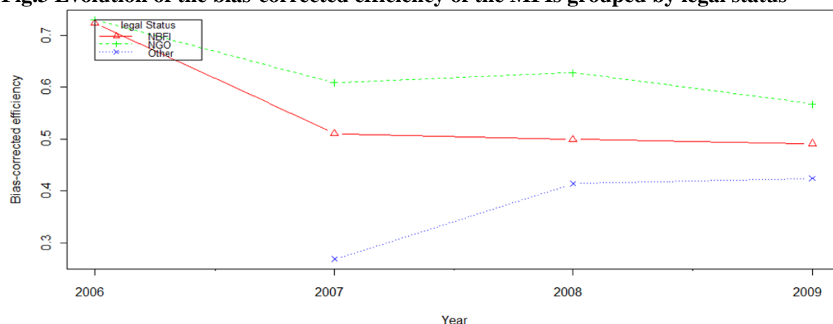
Fig.3 Evolution of the bias-corrected efficiency of the MFIs grouped by legal status
