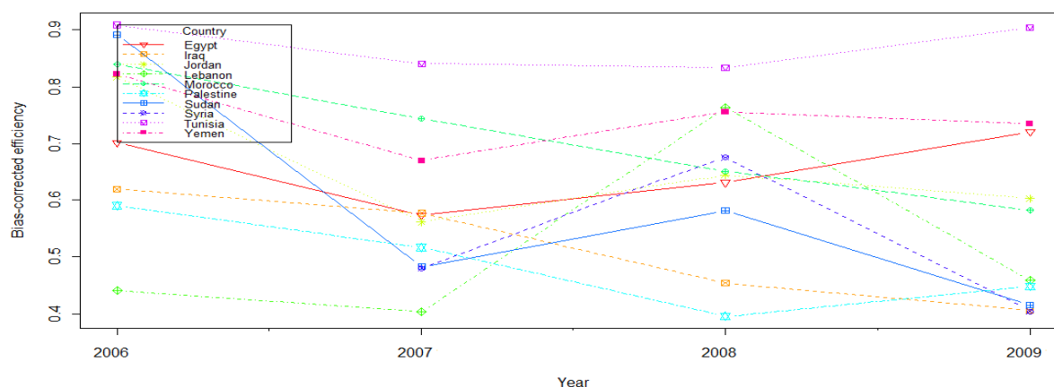
Fig. 2 Evolution of the bias-corrected efficiency of the MFIs grouped by country
