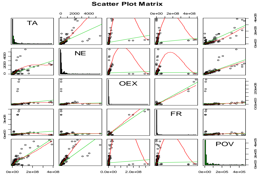
Fig1: Scatterplot matrix of the data set: 3 inputs and 2 outputs, Histogram of the variables on the diagonal.
