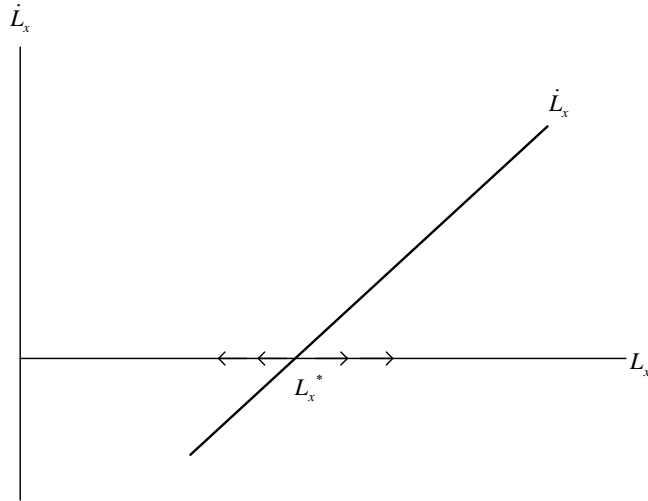
Figure 1. A unique and determinate equilibrium; \theta \rightarrow 0
