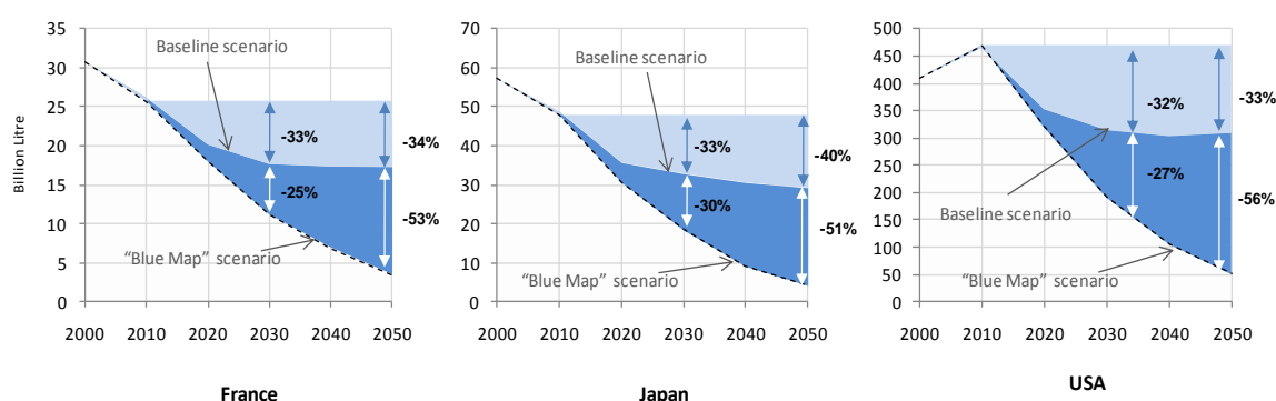
Figure 1. Change in light-duty vehicle gasoline and diesel fuel demand from 2000-2050 under MOMO baseline and “Blue-Map” scenarios: France, Japan and the United States
