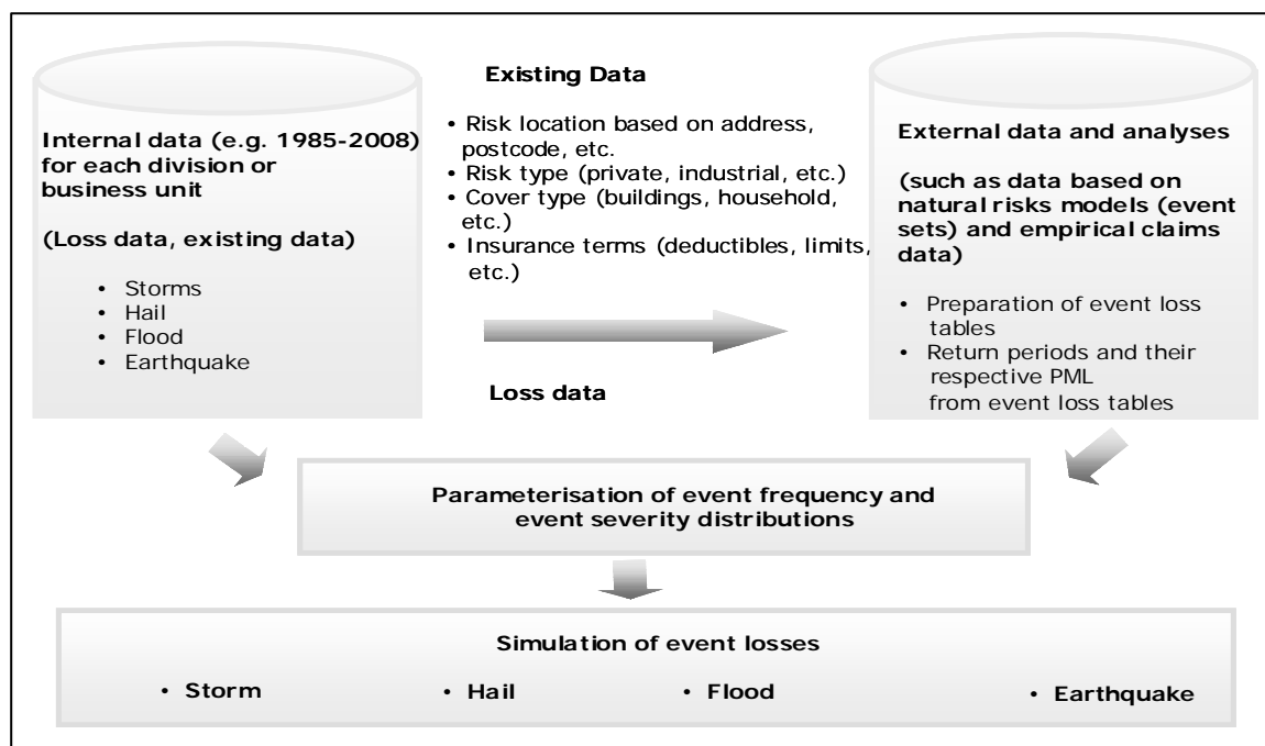
Figure 1: Catastrophe modelling
