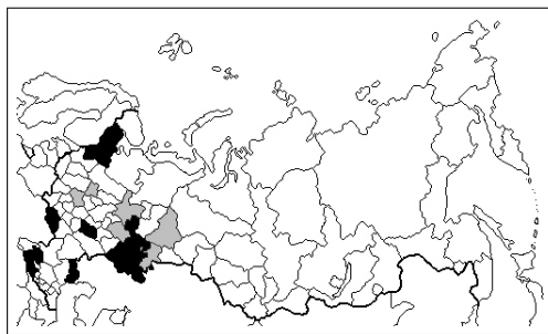
Figure 3: Moran's I - 2004
