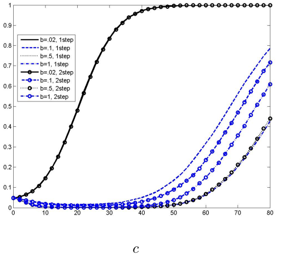
Figure 6: Local Asymptotic Power, Z_t^m , Bartlett Intercept+Linear Trend
