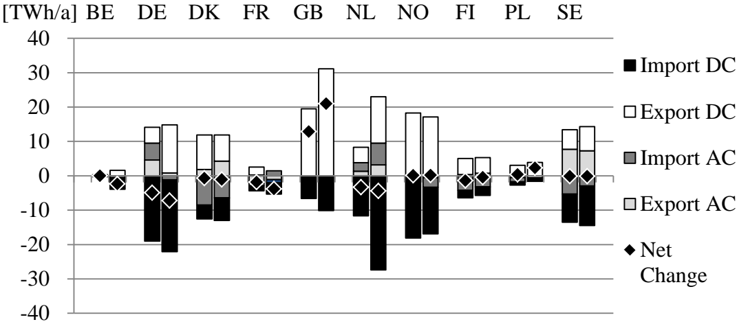
Figure 3: Change in Trade Flows with Trade (left) and Meshed (right) Scenario for 2009 7
