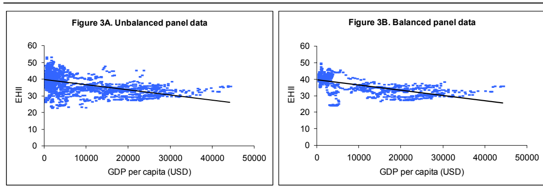
Figure 3. Inequality-growth relationship.
