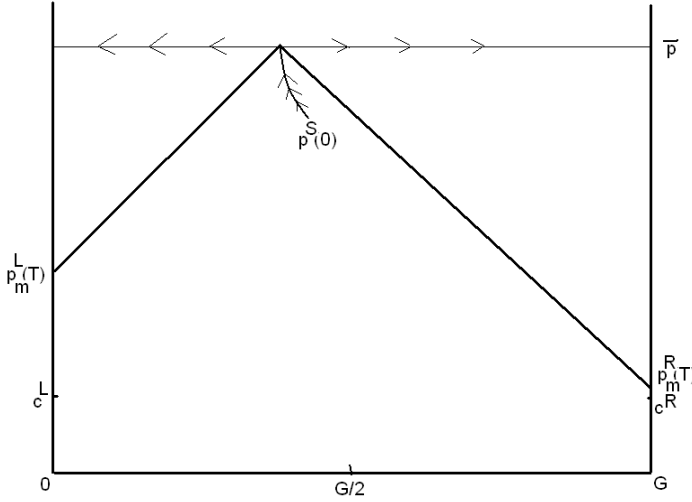
Figure 1: p^S(0) moves up to \bar{p} over Phase I. Each supplier extracts in isolation in Phase II.
