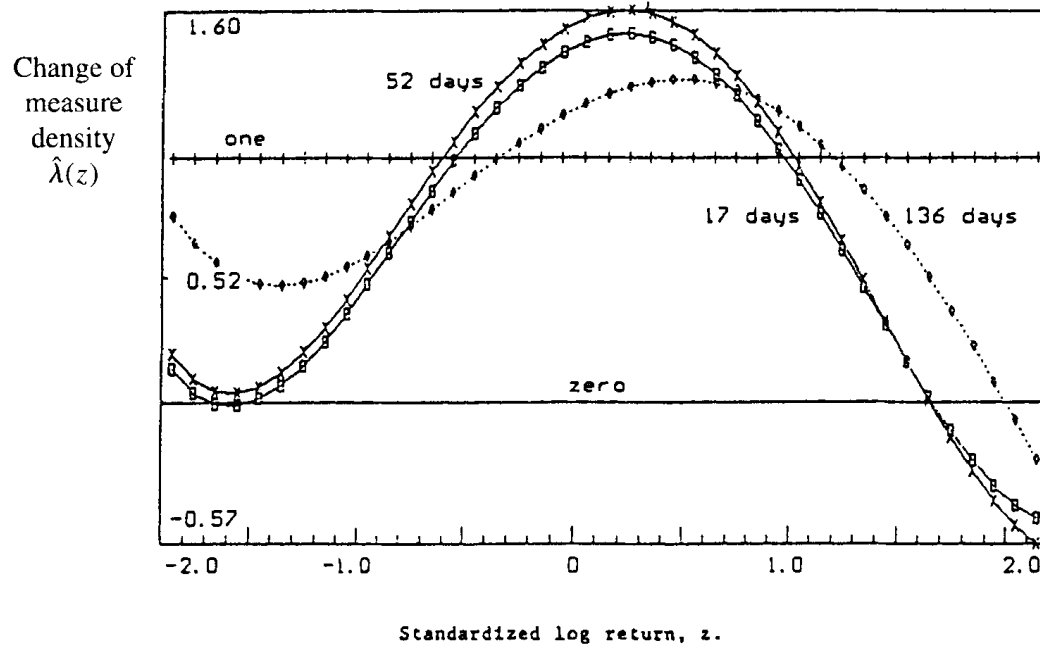
FIGURE 5.1. Equivalent martingale measures for October 31, 1990, maturities of 17, 52, and 136 days.
