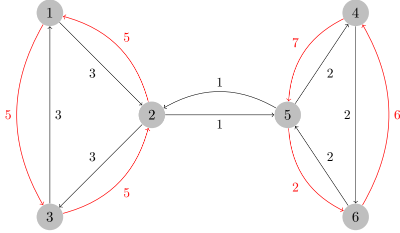
Figure 2: Numeric Version of the Network in Figure 1.
