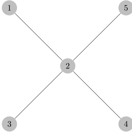
Figure 3: A simple undirected star network.
