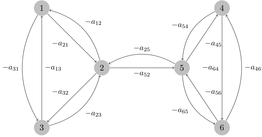
Figure 1: An Example of A Network
