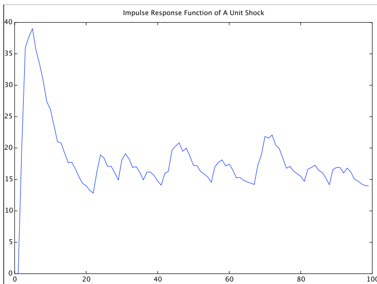
Figure 4: An Impulse Response Function of the Network in Figure 2
