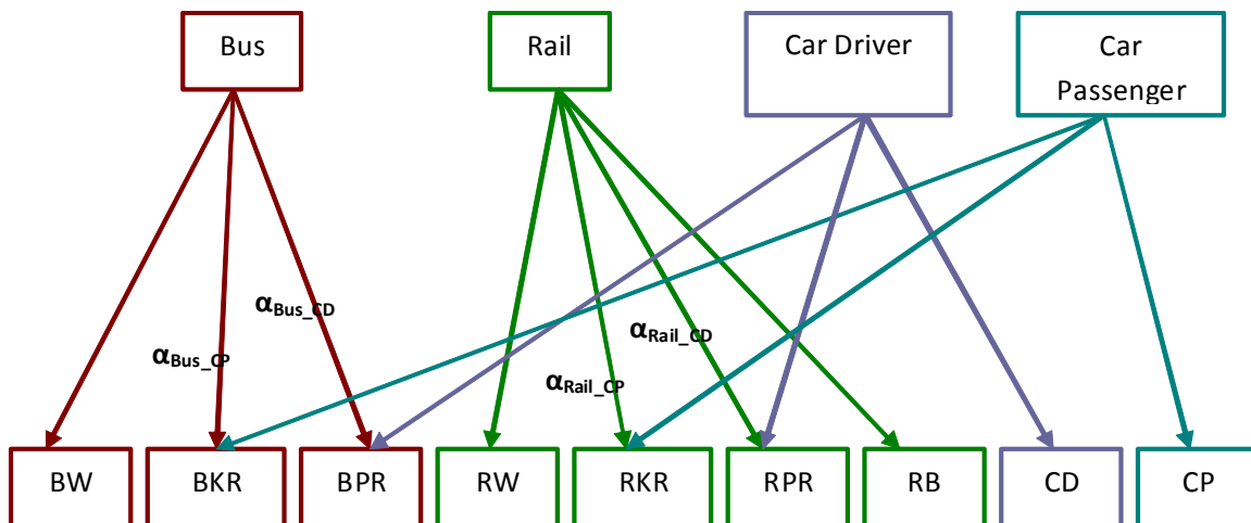
Figure 3. Structure of the Cross-Nested Logit Model
