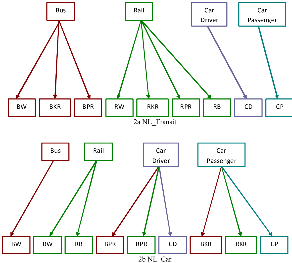
Figure 2. Two Possible NL Structures
