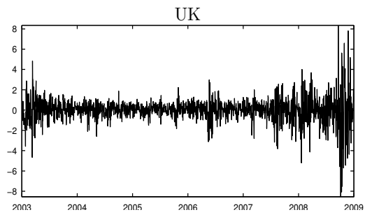
Figure 3. Log-returns of Datastream DS market indices. The number of observations for each series is 1565.
