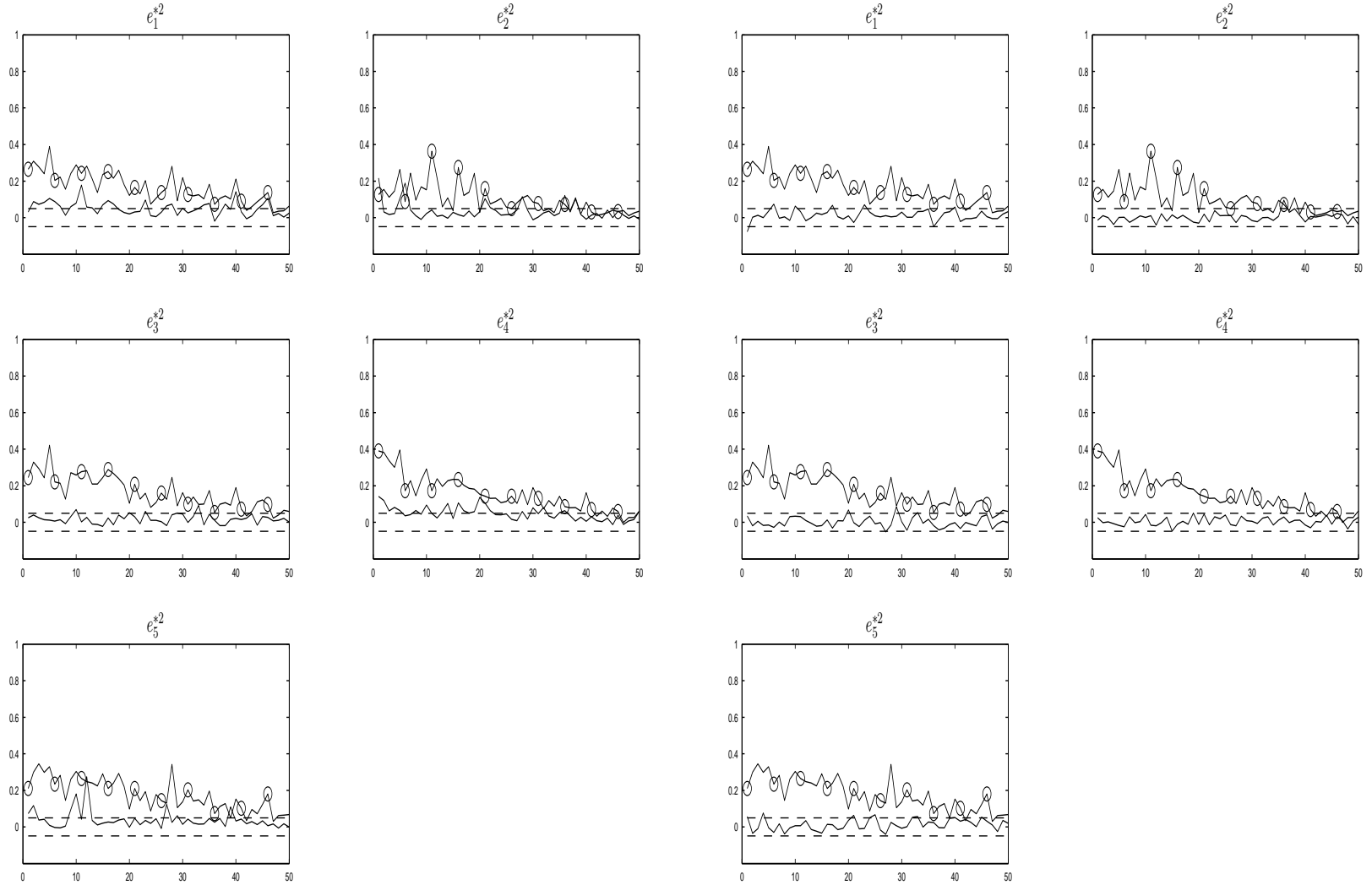
Basic WMSV model
