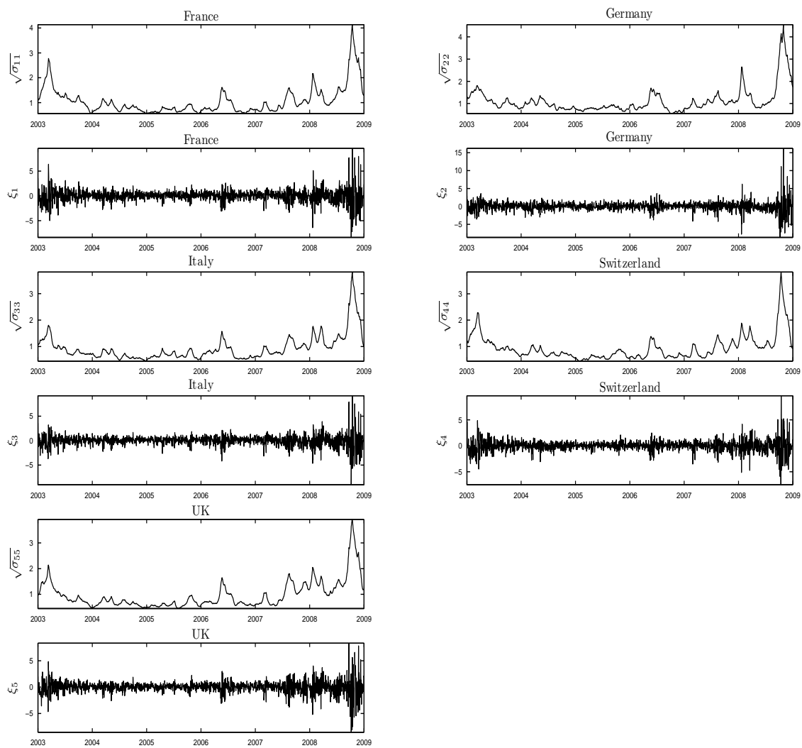
Figure 4. Smoothed volatility estimates and corresponding return series: Basic WMSV model.
