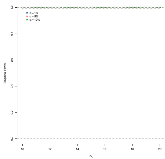
Figure 6: Power curves for exponential random walk II.
