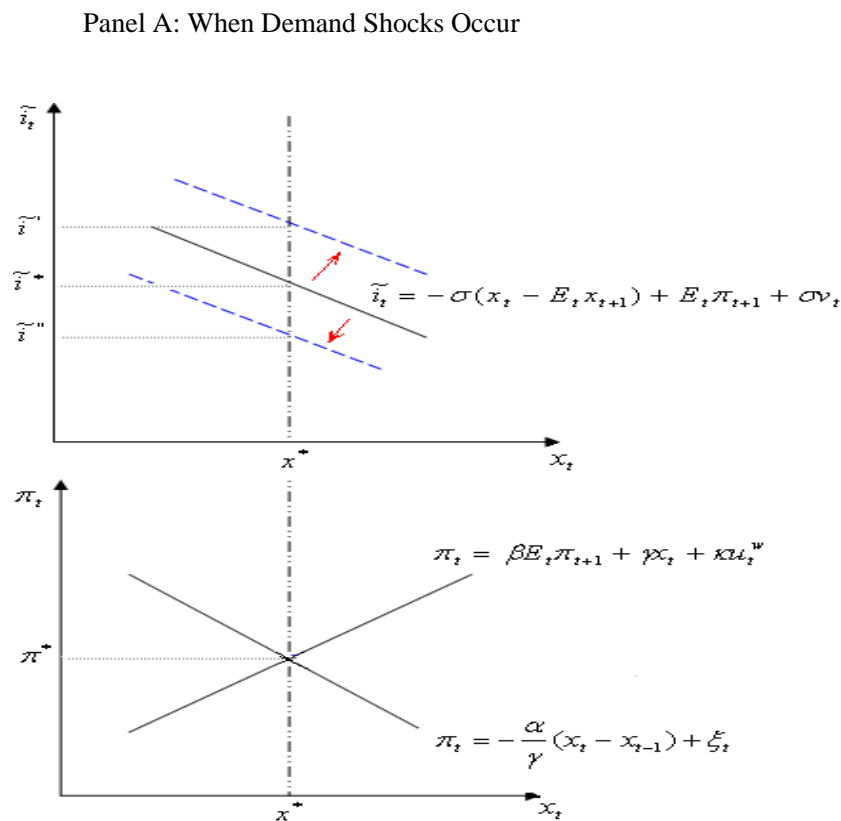
Figure 4.2: Workings of the Baseline Model in Face of Shocks
