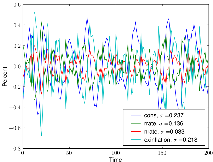
Fig. 3. Baseline Model with habit persistence, prod. shock only
