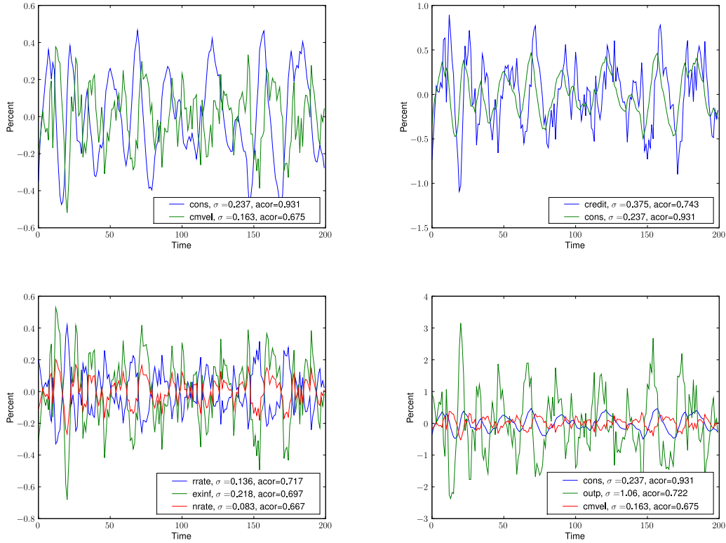
Fig. 2. Baseline Model with habit persistence
