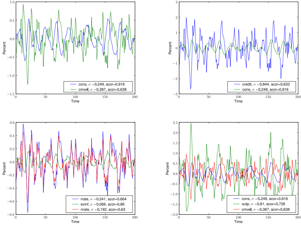
Fig. 4. Baseline Model with habit persistence & adjustment costs
