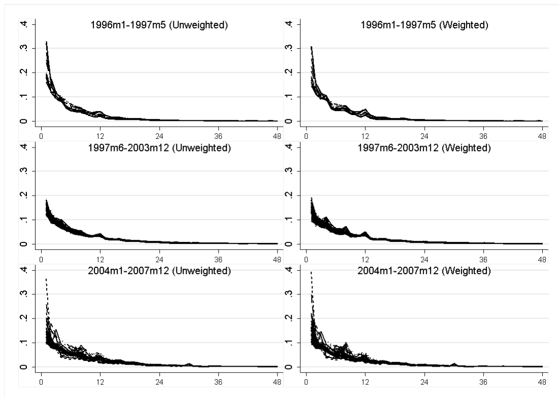
Figure 7 Time-Series Heterogeneity in Distribution of DAF
