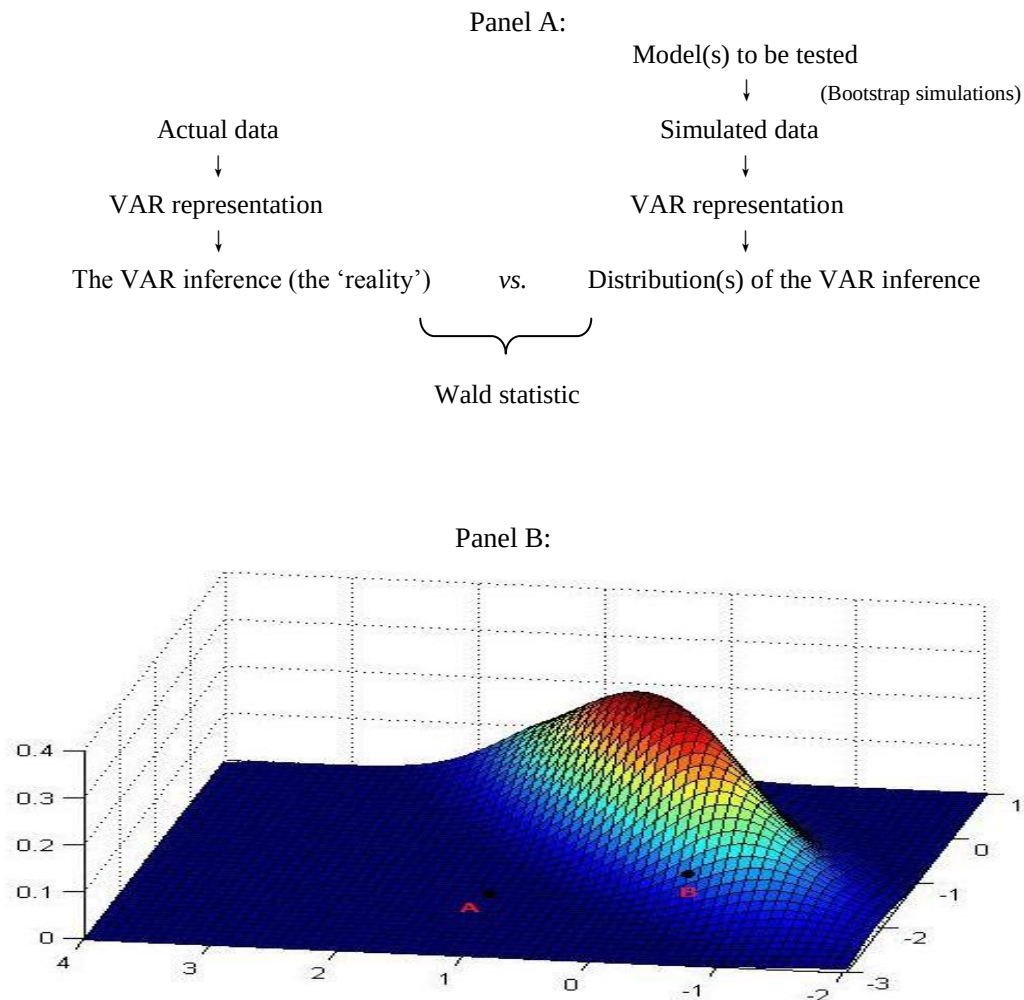
Figure 4.1: the principle of testing using indirect inference
