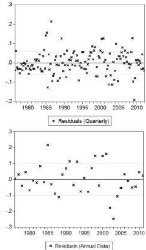
Figure 3: Residual Plots
