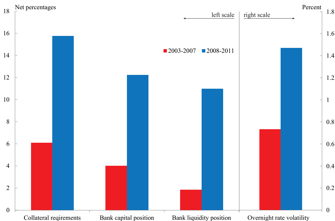
Figure 5: Stylized Facts
