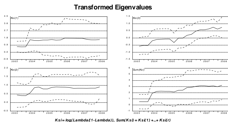
Figure 9: Transformed Eigenvalues
