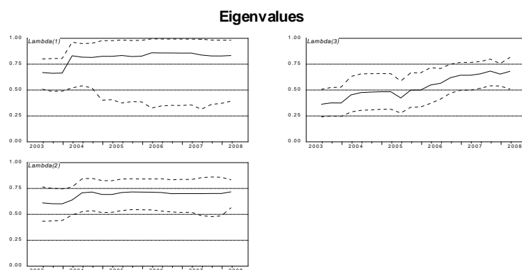
Figure 8: Eigenvalues
