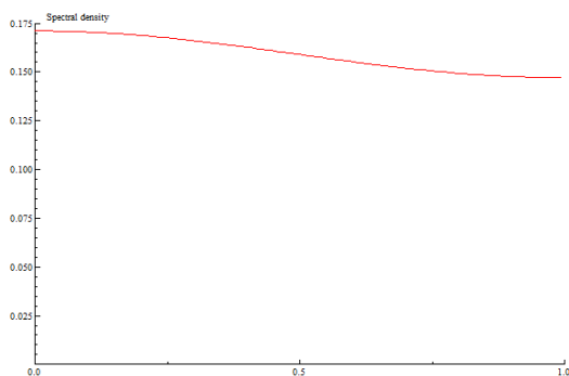
Figure 9: Spectral Density
