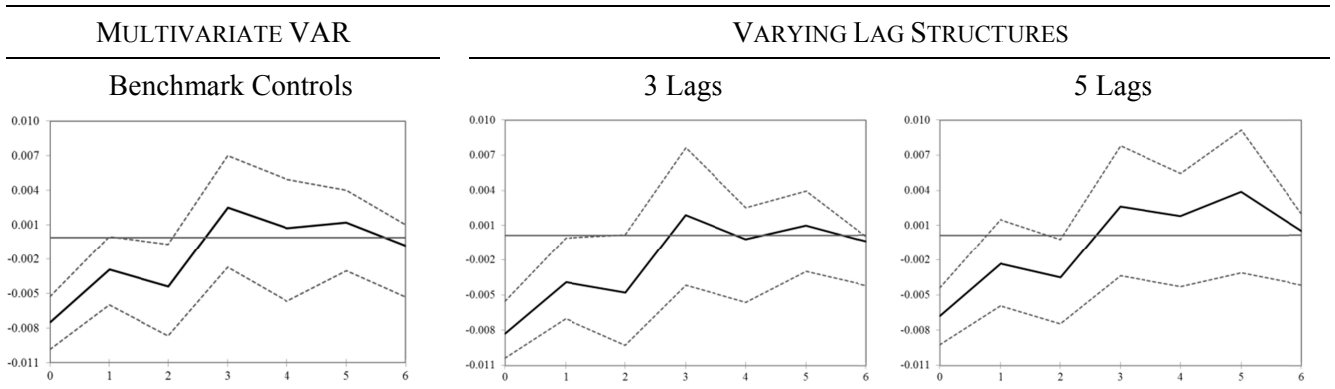
Figure 3: Generalized Impulse Response of Price to Senior Tranche for Different Specifications
