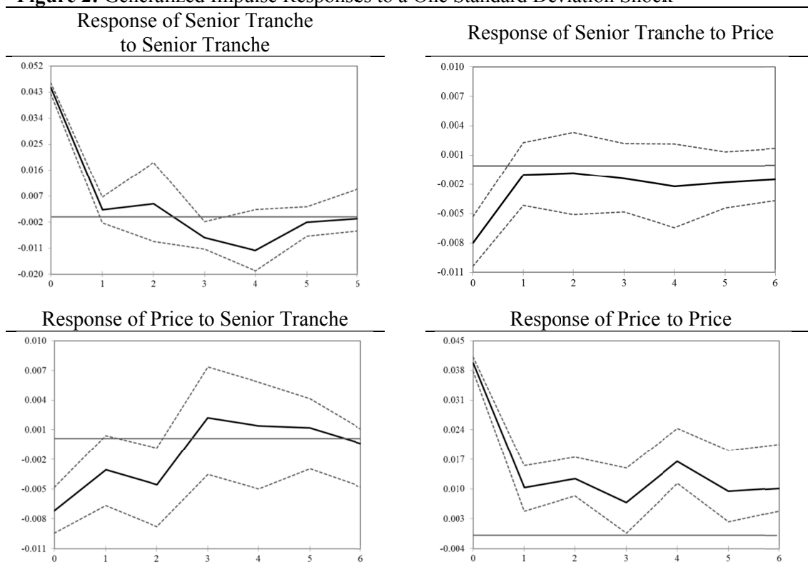
Figure 2: Generalized Impulse Responses to a One Standard Deviation Shock
