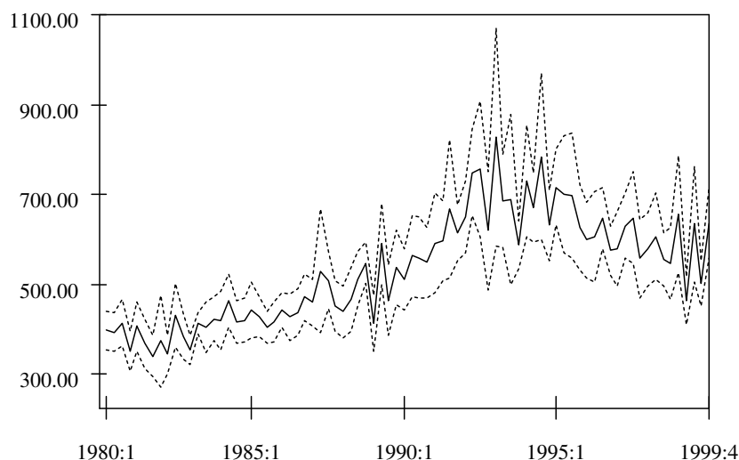
Figure 1: Average price per quarter, units are Deutsche Mark (1 DM \approx 0.511 EURO). Confidence intervals are calculated for the 90% level.
