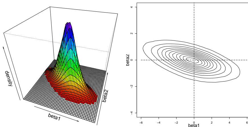
FIGURE 13. Parametric Normal random coefficients model estimate of the bivariate density of (\beta_{i1}, \beta_{i2}) .
