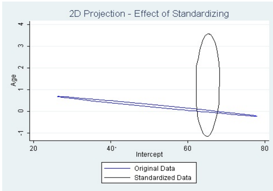
Figure 1: H(\theta) and H(\hat{\theta}) obtained, respectively, using x_{-1} and \frac{x_{-1} - \mathbf{E}(x_{-1})}{\sqrt{\mathbf{Var}(x_{-1})}} .
