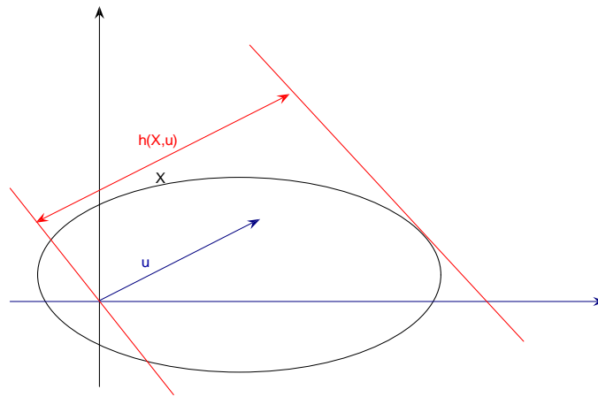
Figure 2: Support function of X at u .
