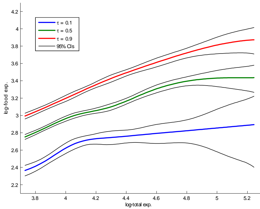
Figure 8: RP Constrained quantile Engel curve estimates, t = 1983 .
